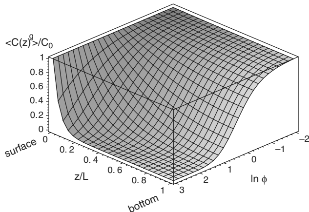
Fig. 6 Oxidant concentration inside the porous medium as a function of Thiele number.
